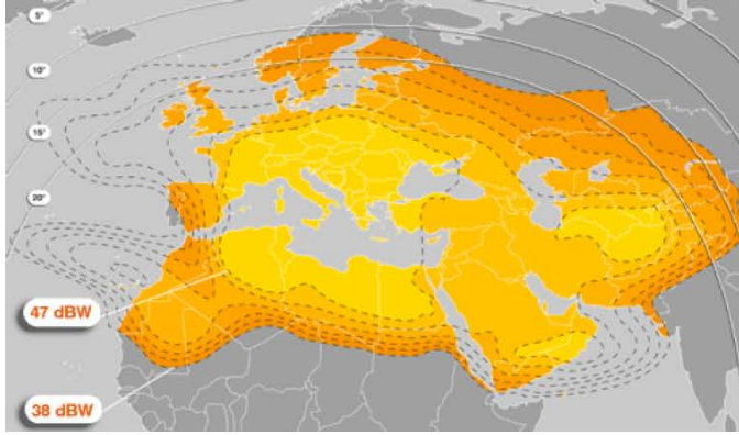
Eutelsat W6 coverage, 21.5° East
